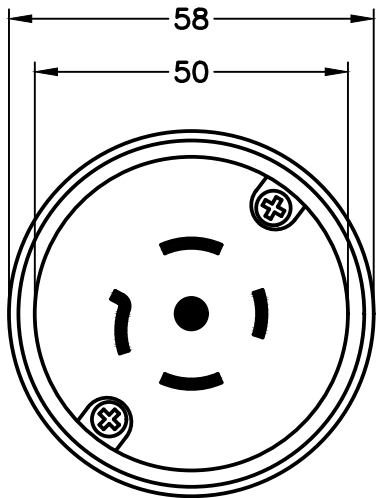
NEMA L21-20 PLUG FRONT VIEW
